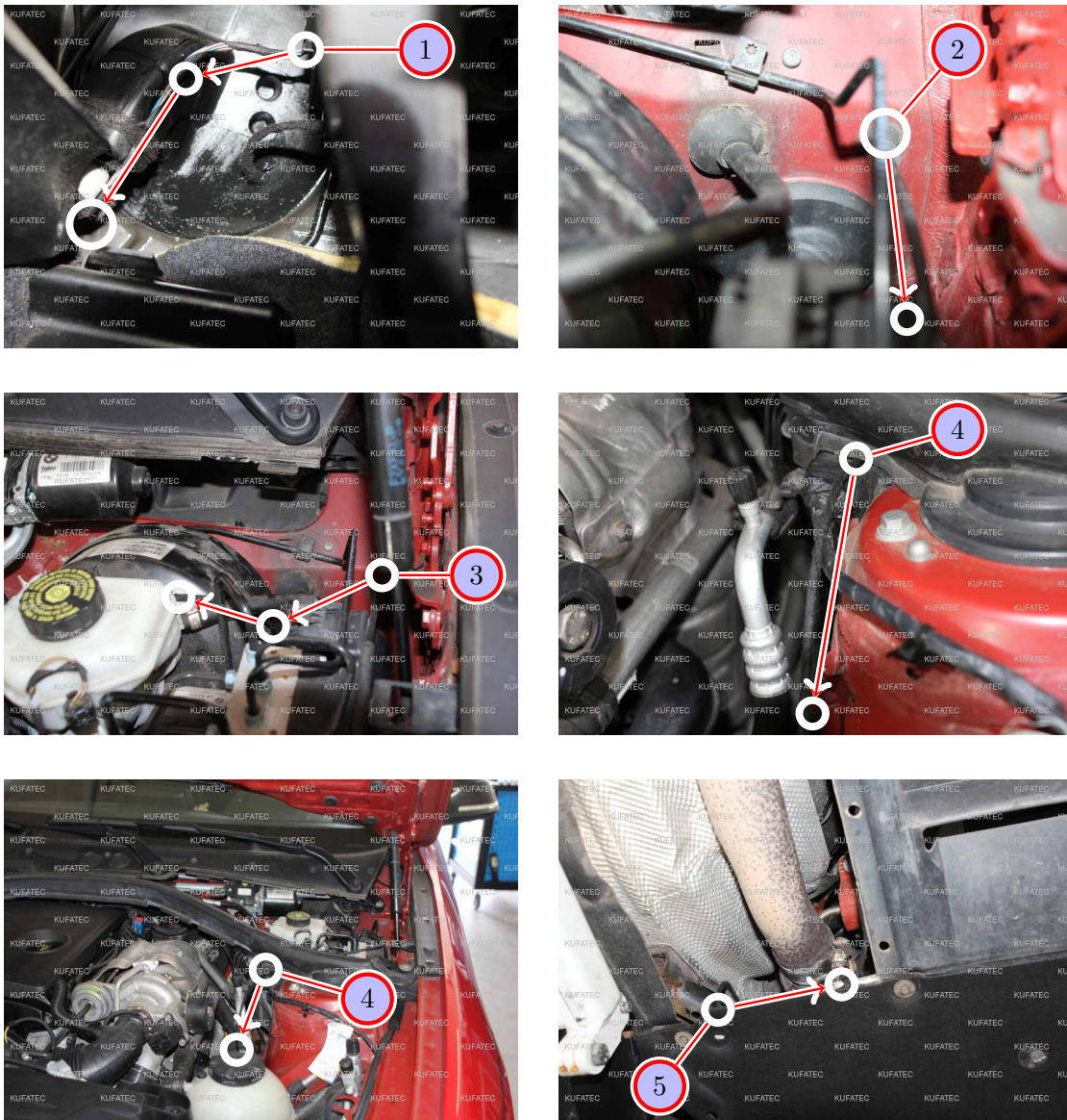
Figure 6: Cable routing to the sound generator
