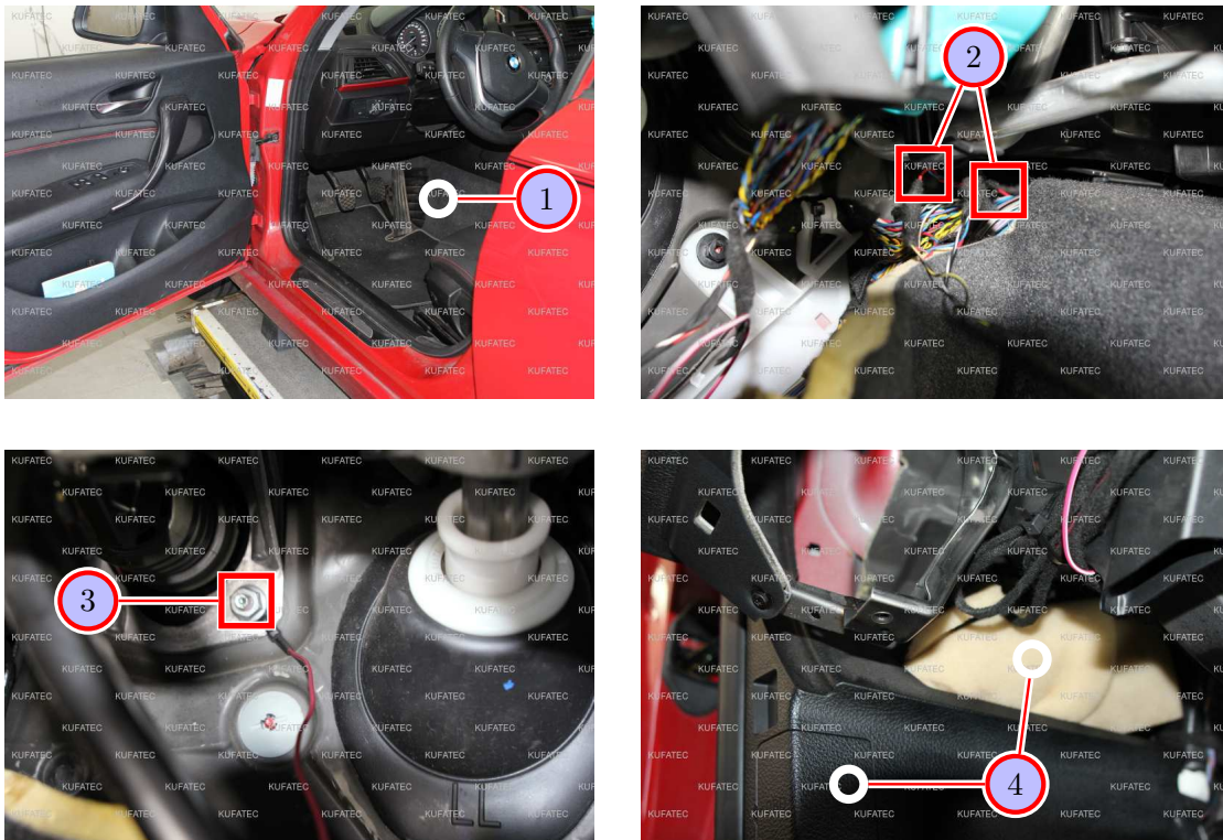
Figure 5: Connection Can High & Low / Ground
