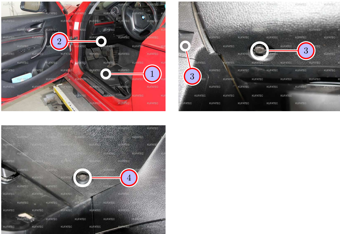
Figure 4: Removing trim panel of the dashboard on driver's side
